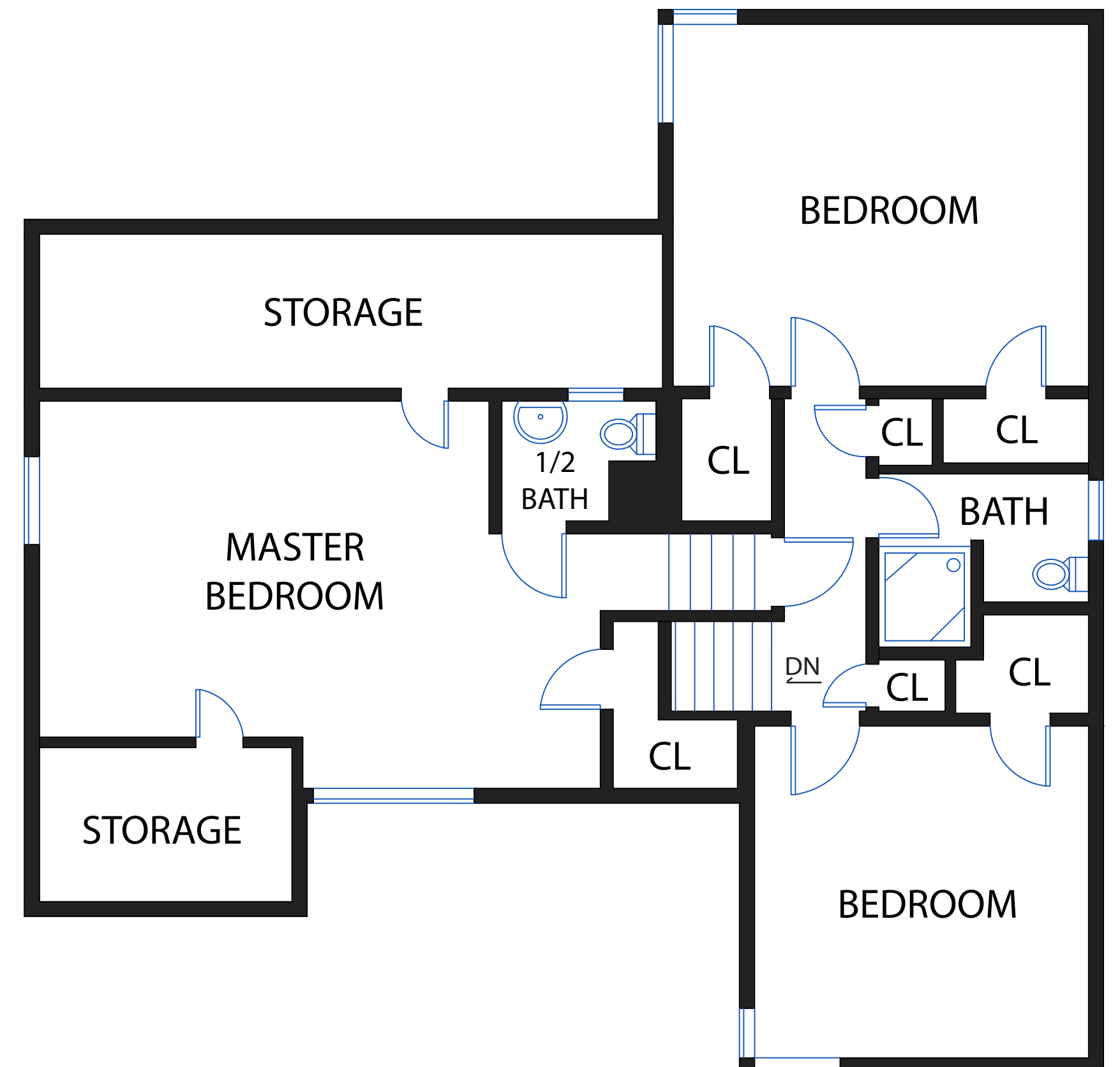
UPPER LEVEL
